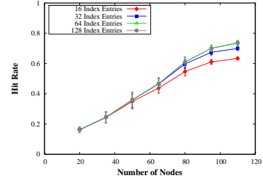
Figure 20. Mobile IM with integrated approach: system size vs. hit rate
